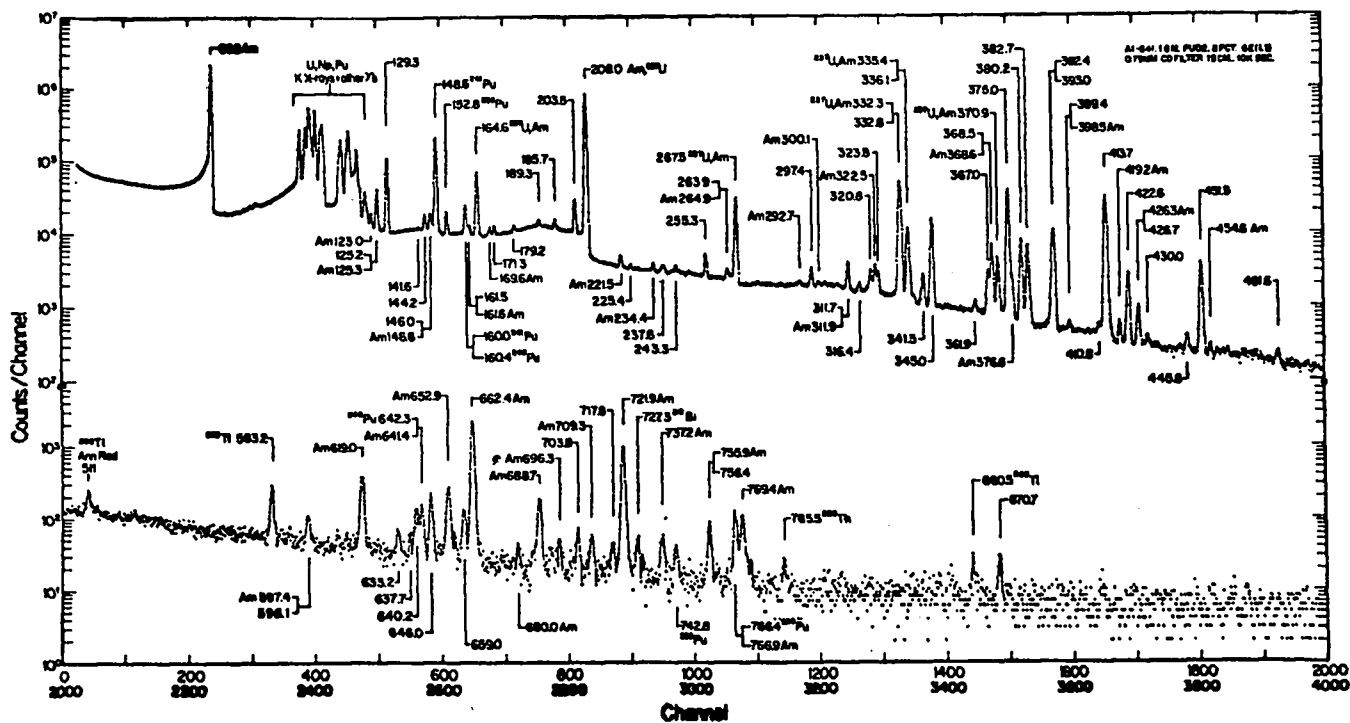
Fig. 12. 1-g PuO 2 , 8% Ge(Li) with 0.8-mm Cd filter. Source distance is 15 cm. Count time is 10 4 seconds.
