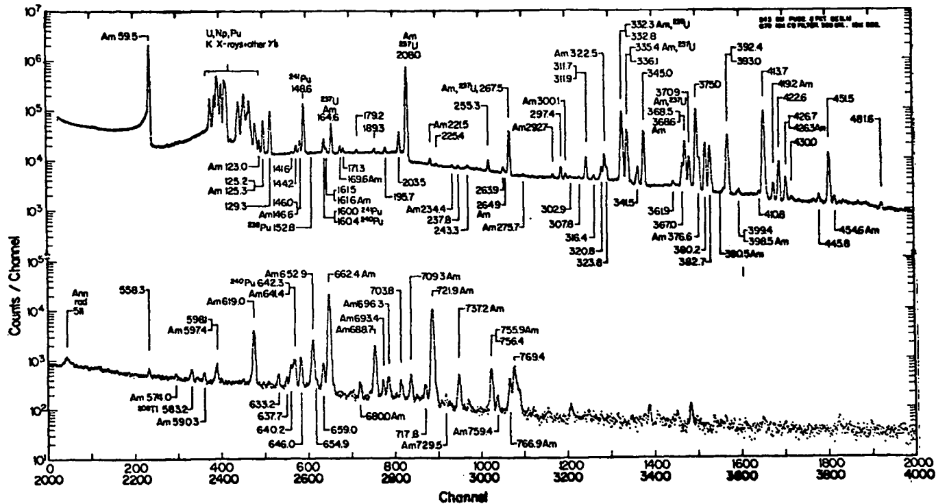
Fig. 13. 543g PuO 2 , 8% Ge(Li) with 0.8-mm Cd filter. Source distance is 1 m. Count time is 10 4 seconds.
