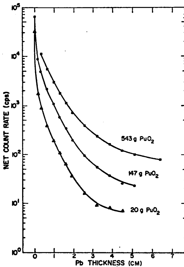
Fig. 3. Broad-Beam Attenuation from PuO 2 Samples.
